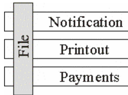
Figure 3. File dependencies.
