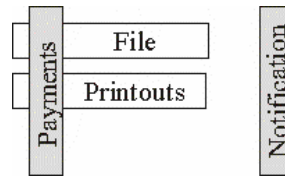
Figure 5. Payments dependencies.
