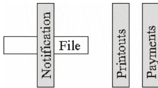
Figure 2. Notification dependencies.
