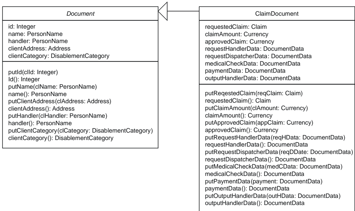
Figure 2. Part of the document class hierarchy, which is used for representing client requests.
