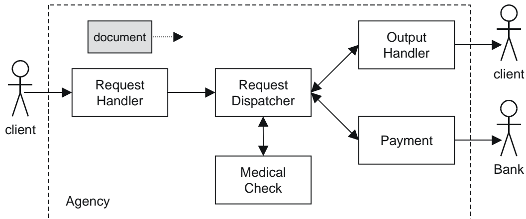
Figure 1. Tasks in the example system.
