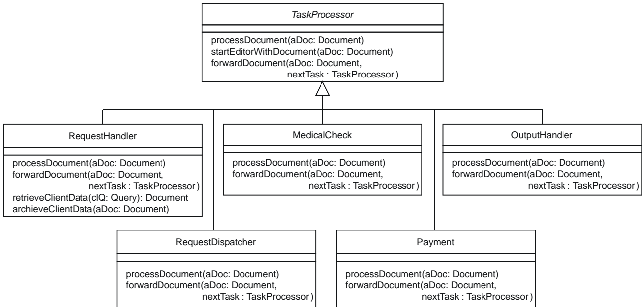
Figure 3. Class hierarchy for tasks.
