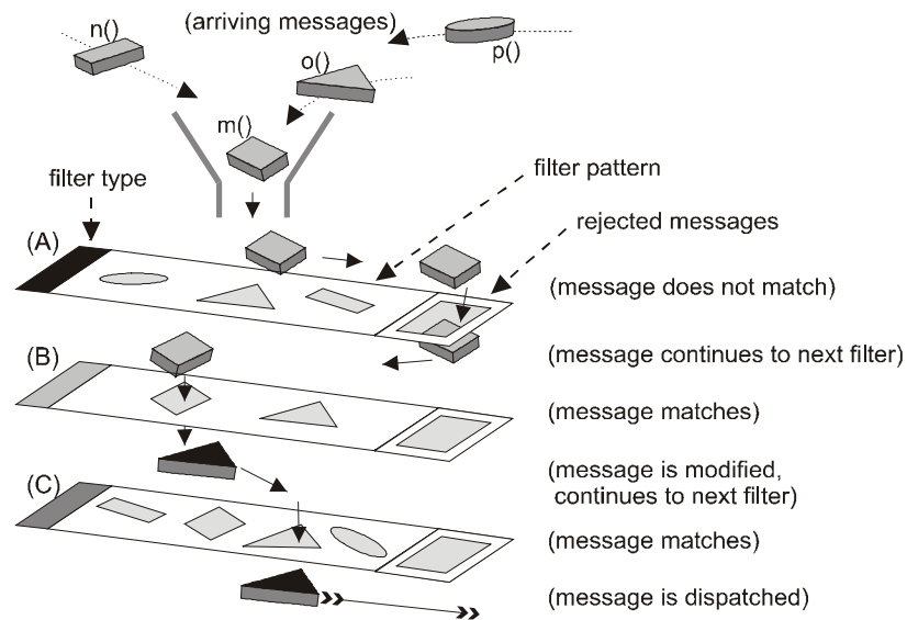
Figure 7. An intuitive schema of message filtering.
