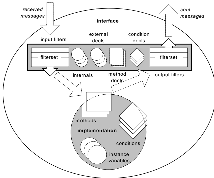
Figure 5. Simplified representation of the CF model.
