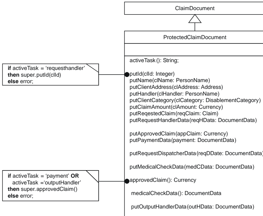
Figure 4. Class ProtectedClaimDocument with the pseudo-code implementations of putId and approvedClaim.
