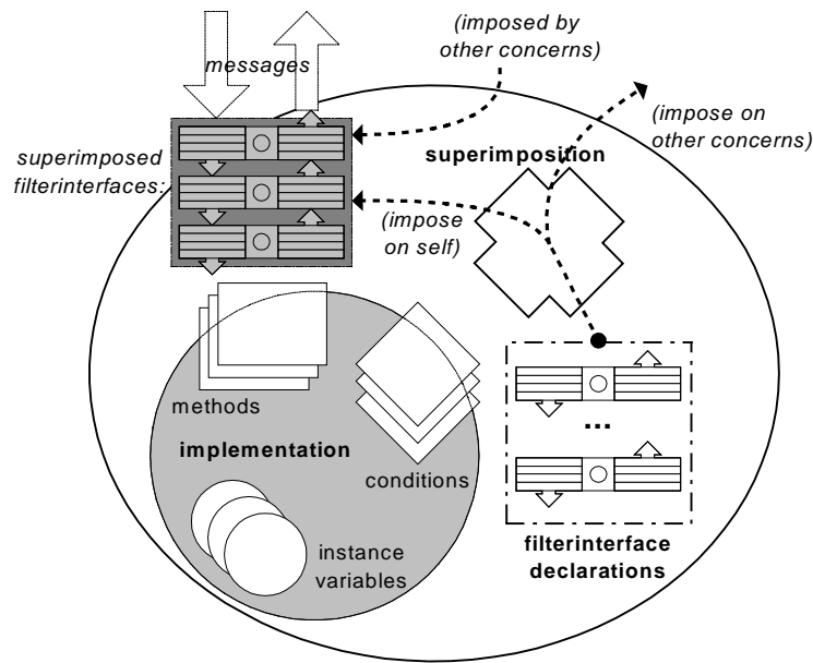
Figure 8. The CF model with superimposition.
