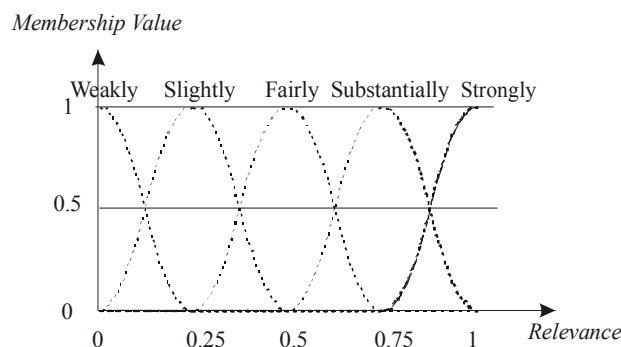
Fig. 3. Definition of linguistic variable Relevance.
