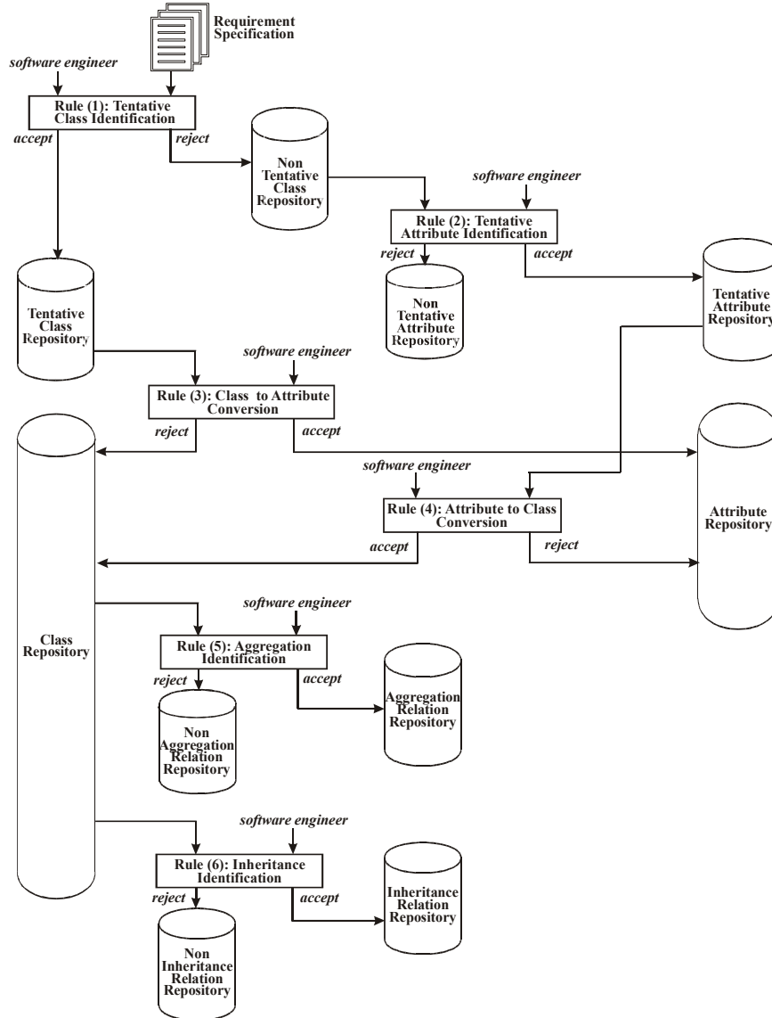
Fig. 1. The casual dependencies between the rules of the example method.
