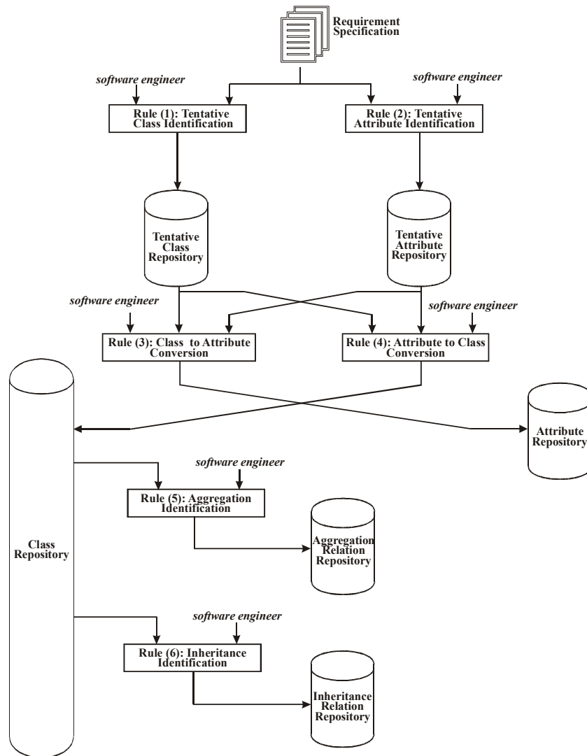
Fig. 5. The casual dependencies between the rules of the fuzzy example method.
