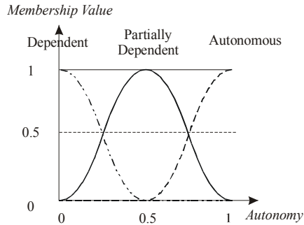
Fig. 4. Definition of linguistic variable Autonomy.
