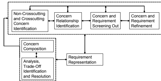
Figure 2: A General Process for AORE
