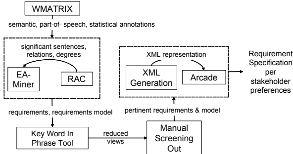
Figure 3: Tool Suite for AORE
