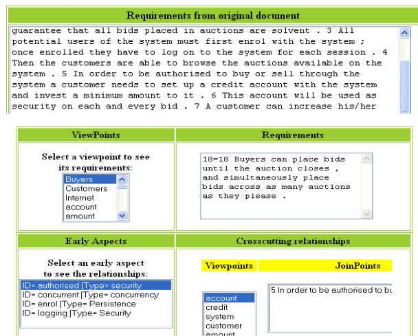
Figure 7: EA-Miner tool
