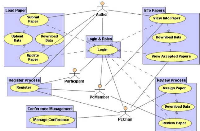
Figure 3. Use case model of the Conference Review System
