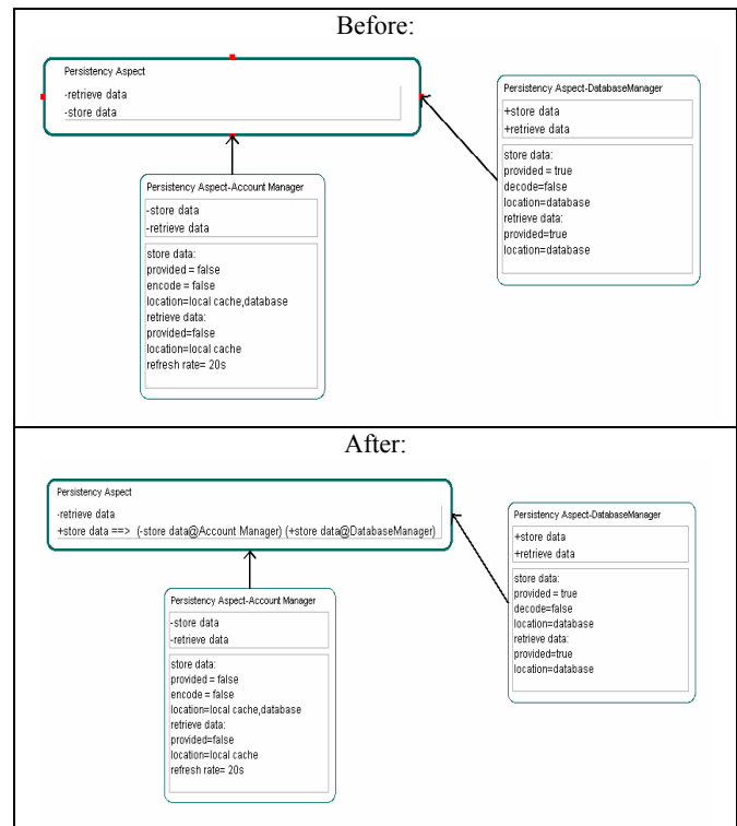
Figure 9: The aspect diagram for the persistency aspect before and after being mapped.
