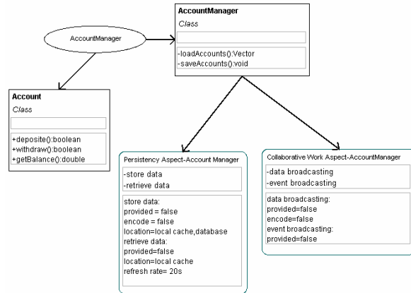
Figure 8: The component diagram of AccountManager.
